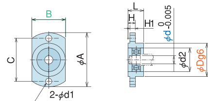
Supported side
