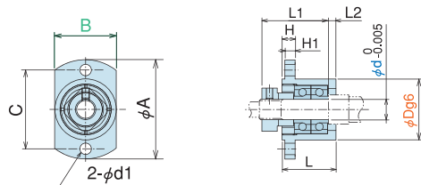
Round type fixed side Support unit
