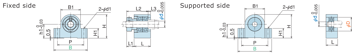
Square type fixed side Support unit
