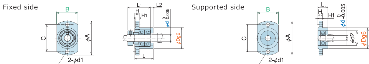
Round type fixed side Support unit
